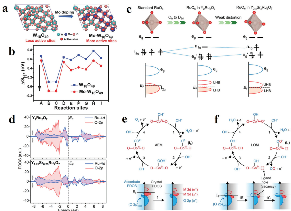
Fig. 10 (a) Different oxygen sites on W_{18}O_{49} (010) and Mo-W_{18}O_{49} (010). (b) The calculated Gibbs free energy of HER on different oxygen sites of W_{18}O_{49} (010) and Mo-W_{18}O_{49} (010). 113 (c) Schematic illustrations of different RuO_6 along with the splitting of Ru 4d orbitals. (d) Schematic evolution of band alignments through Sr^{2+} substitution for Y^{3+} in Y_2Ru_2O_7 . 127 (e and f) Relationship between oxygen vacancy concentration and Co–O bond. 115
