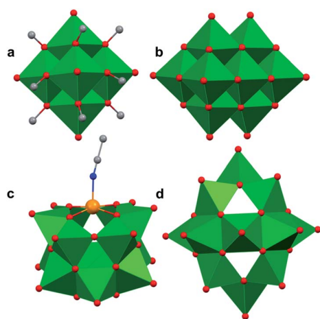
Fig. 1 Popular structures of POV clusters: (a) [\text{V}_6\text{O}_7(\text{OCH}_3)_{12}]^{1-} , (b) [\text{V}_{10}\text{O}_{28}]^{6-} , (c) [\text{V}_{12}\text{O}_{38}\text{Co}]^{2-} , and (d) [\text{H}_2\text{V}_{18}\text{O}_{44}(\text{N}_3)]^{5-} . Colour code: V: green polyhedra, O: red, C: grey, N: blue, Co: orange. Hydrogen atoms, solvent molecules and counter cations are omitted for clarity.
