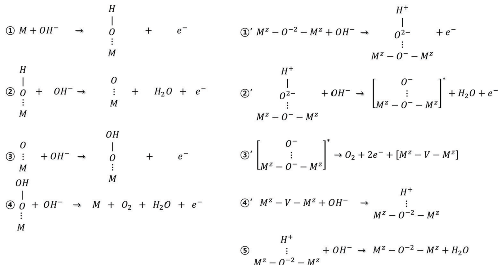
Fig. 1 Perovskite catalysts are plausible to undergo both conventional and lattice oxygen participating mechanisms as sketched in (a) and (b), respectively. 1 The conventional mechanism consists of concerted proton electron transfers while step 3' of the lattice oxygen participating mechanism is a decoupled transfer of charges. (c) The dissolution of surface cations is another competing reaction which the catalyst may undergo due to the thermodynamic instability under the oxygen evolution reaction condition.
