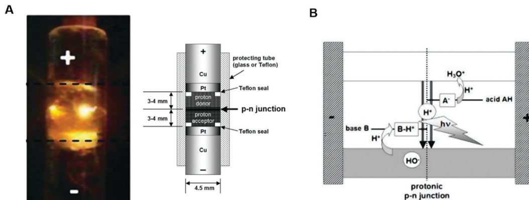
Fig. 6 (A) Dx50/Dx1 based protonic light emitting diode. Inset shows the schematic of the device; (B) scheme of the light emission in the middle of the junction under the application of a forward bias (i.e. a positive voltage at the proton donor/Pt electrode interface). (Reproduced and adapted from ref. 11, copyright (2020), Royal Society of Chemistry (RSC)).
