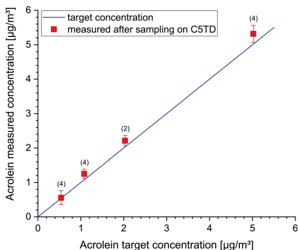
Fig. 4 Acrolein target concentrations in the air of an empty 1 m 3 glass test chamber versus acrolein concentration measured after active sampling on Carbograph TM 5TD (C5TD). The whiskers show the respective standard deviations, the numbers in brackets indicate the number of repeated measurements. Individual data (target/measured in µg m -3 ): 0.54/0.56 ± 0.21; 1.08/1.25 ± 0.14; 2.03/2.21 ± 0.15; 5.02/5.31 ± 0.25.
