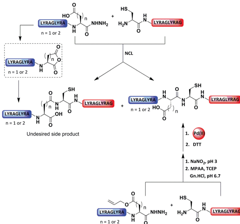
Fig. 12 \text{Pd(II)} -Mediated removal of allyl PG after the ligation at Asp/Glu for peptide synthesis.
