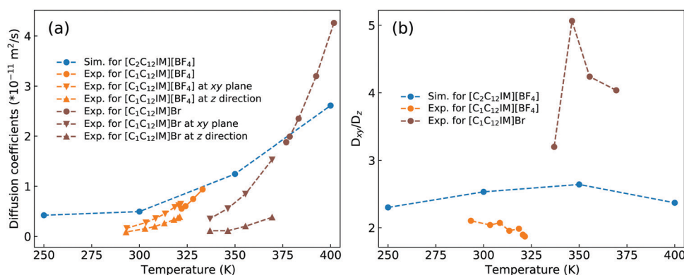
Fig. 15 Comparison of (a) the total diffusion coefficient data and (b) the fractions of in-plane diffusion coefficients ( D_{xy} ) over those along z -axis ( D_z ) of [C_2C_{12}IM] cations in [C_2C_{12}IM][BF_4] IL obtained from current CG MD simulations with experimental measurements of [C_1C_{12}IM][BF_4] IL at relevant temperatures. 83 The experimental data for [C_1C_{12}IM]Br IL at different temperatures are also provided for a comparative purpose. 84
