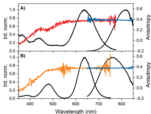
Fig. 2 Overlay of steady-state excitation (red and orange) and emission anisotropy (blue) together with the vertical-vertical (VV) excitation (black) and VV emission spectra (black). 23 The detector used on the FluoTime300 has a limited sensitivity above 800 nm, and hence the spectral shape becomes increasingly unreliable with increasing wavelength. However, anisotropy is a ratiometric quantity and thus not affected by this. (A) DNA841-AgNCs and (B) DNA811-AgNCs in 95% glycerol and 5% 10 mM NH 4 OAc aqueous solution at 5 °C. See Fig. S5 (ESI†) for additional measurement details.
