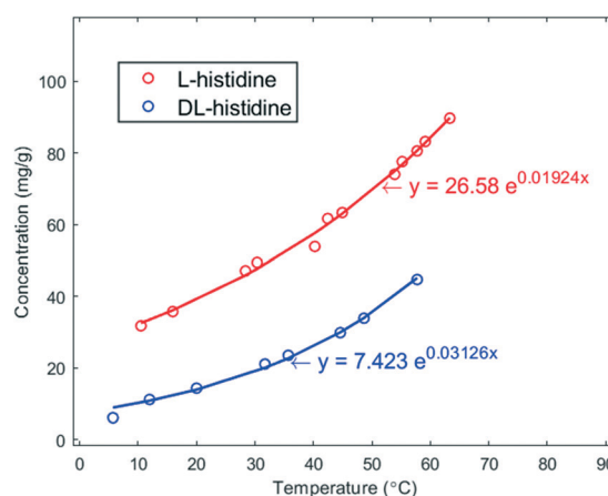
Fig. 1 Solubility curves in \text{mg g}^{-1} of L- (red) and DL-histidine (blue) in water as a function of temperature in ^{\circ}\text{C} . The solid lines are fits of the data.
