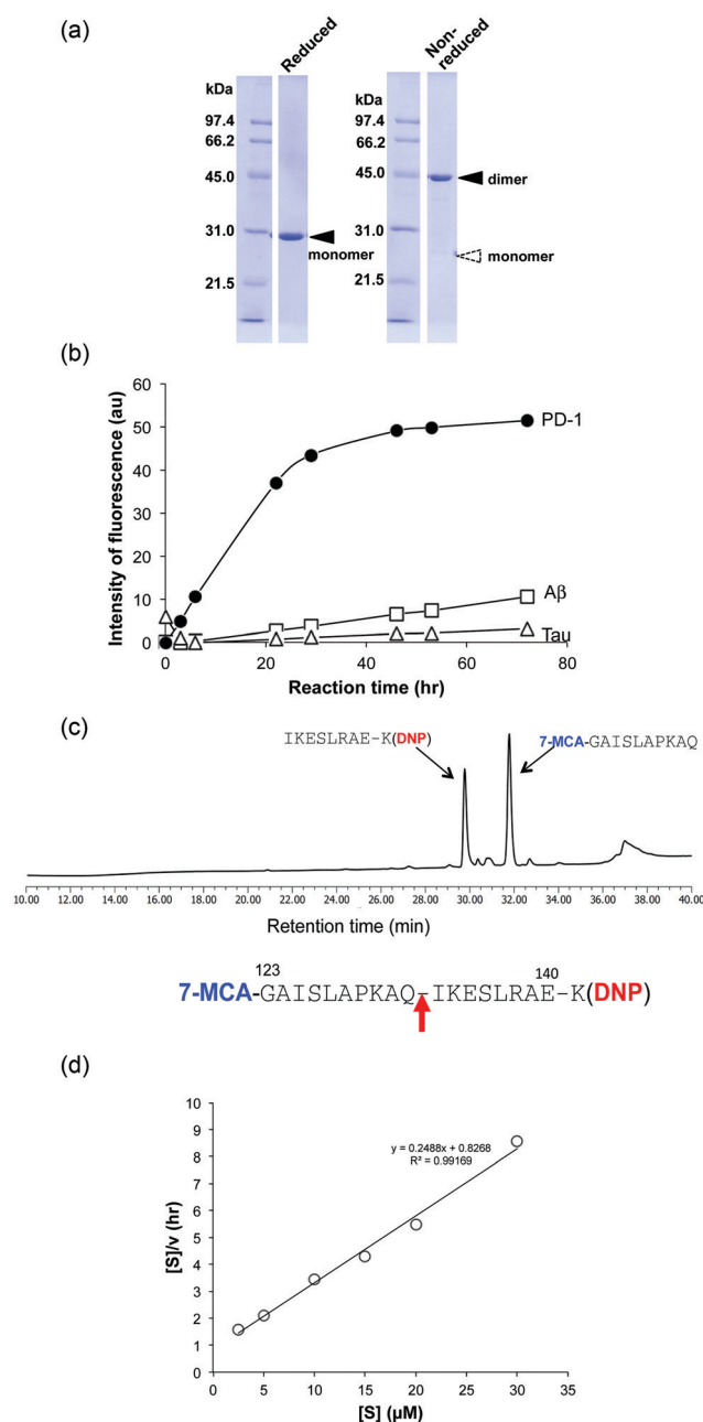
Fig. 2 (a) Results of SDS-PAGE analysis: a band of the dimer at \sim 44 kDa is observed under non-reduced conditions. Under reduced conditions, only a single \sim 29 kDa band corresponding to the monomer is detected. Bands other than the monomer of the light chains were essentially absent under either reducing or non-reducing conditions. (b) Cleavage reaction for FRET substrates: the cleavage reaction was performed with 5 \mu M H34 using 25 \mu M of FRET-PD1 (PD-1; aa 123–140), FRET-A \beta (A \beta ; aa 26–33) or FRET-Tau (Tau; aa 391–408). H34 exhibited strong catalytic activity for FRET-PD1, but low activity on FRET-A \beta or FRET-Tau. All reactions were carried out in duplicate. (c) Bond cleavage for FRET-PD1: the H34 reaction products were analyzed by HPLC and MS. The fragments were identified as 7-MCA-GAISLAPKAQ-OH (31.7 min) and NH 2 -IKESLRAEK(DNP)-NH 2 (29.6 min), indicating cleavage of the peptide bond between Gln132 and Ile133. (d) Kinetic analysis: [S]: concentration of the FRET-PD1 substrate. [V]: initial rate of the cleavage reaction. The Hanes–Woolf plot demonstrates that cleavage by the H34 light chain fits Michaelis–Menten kinetics, indicating that the reaction is enzymatic. k_{\text{cat}} and K_{\text{m}} were 1.3 \times 10^{-2} \text{ min}^{-1} and 3.32 \times 10^{-6} \text{ M} , respectively.
