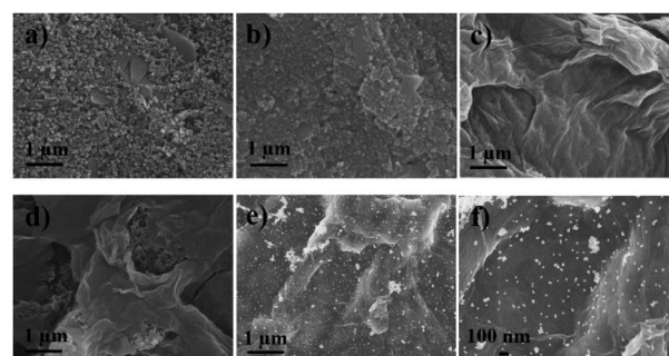
Fig. 2 SEM images of (a) SPCE, (b) GQDs/SPCE, (c) GO/SPCE, (d) GQDs/GO/SPCE, and AuNPs/GQDs/GO/SPCE with (e) low magnification (x20 000) and (f) high magnification (x50 000). The bright spots or small particles in (e) and (f) are AuNPs.
