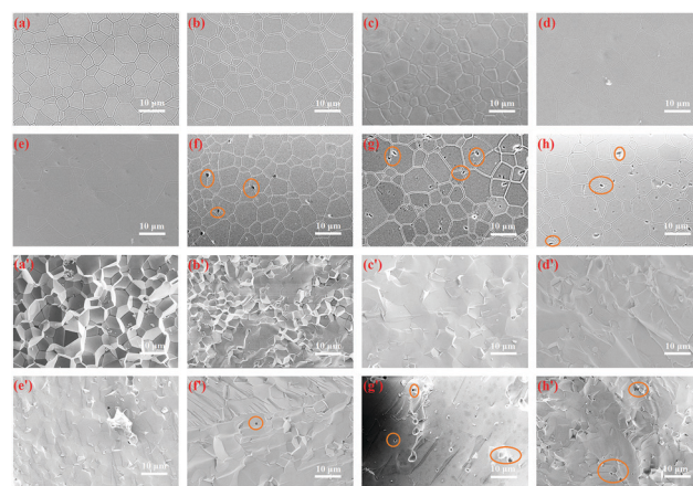
Fig. 2 SEM images of the thermal etched surfaces and the fracture surfaces of (a) and (a') Pr0Mn0, (b) and (b') Pr02Mn0, (c) and (c') Pr0Mn04, (d)–(h) and (d')–(h') Pr005Mn05, Pr01Mn06, Pr015Mn07, Pr02Mn08, and Pr04Mn10.
