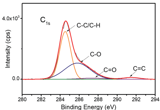
Fig. 4 XPS spectrum of P(VGal 10% -co-St 90% ) remained on fractured surface after adhesion tests.
