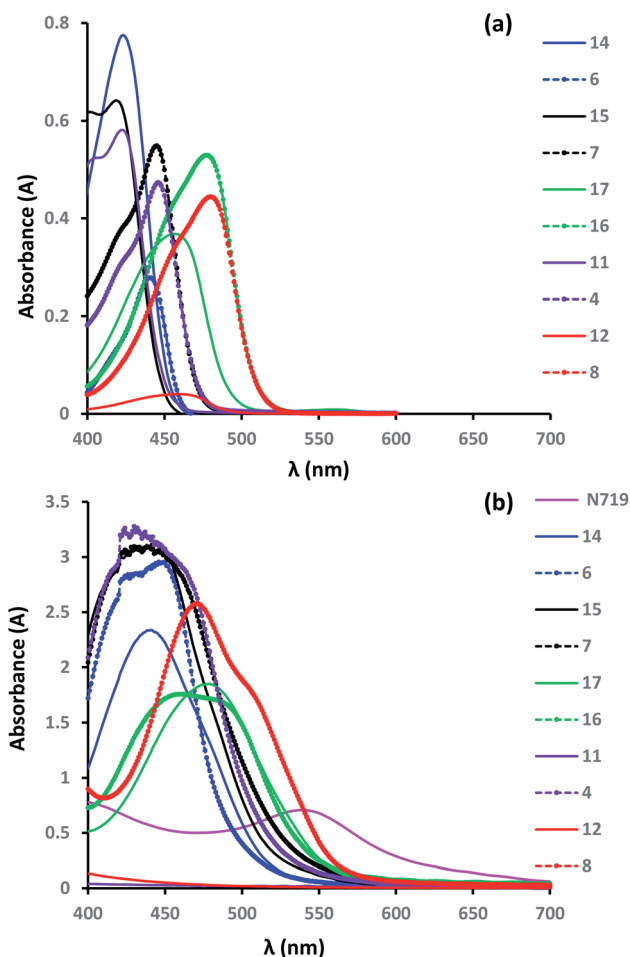
Fig. 2 UV-Vis spectra of (a) HfsQ dyes in solution and (b) dyes adsorbed onto a transparent \text{TiO}_2 surface. For clarity, structurally related dyes have same colour and \text{C}(\text{CH}_3)_2 dyes have solid lines, whilst S dyes have dashed lines with circle markers.
