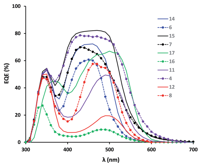
Fig. 4 EQE of DSC devices using HfSQ dyes. For clarity, structurally related dyes have same colour and \text{C}(\text{CH}_3)_2 dyes have solid lines, whilst S dyes have dashed lines with circle markers.
