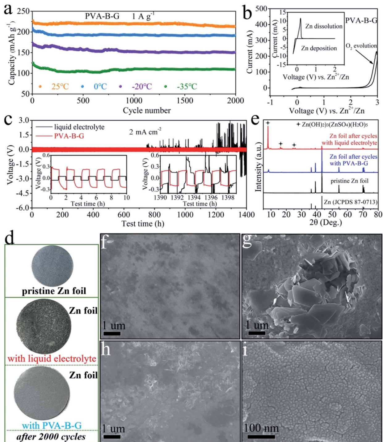
Fig. 5 (a) Cycling performances of the PVA-B-G battery at 1 \text{ A g}^{-1} at different temperatures. (b) CV curve of Zn deposition/dissolution in a \text{Zn} // \text{PVA-B-G} // \text{stainless steel} cell between -0.2 and 3.0 \text{ V} . (c) GCD curves of \text{Zn} // \text{Zn} symmetrical cells with PVA-B-G and liquid electrolytes cycled at 2 \text{ mA cm}^{-2} (insets show the enlarged voltage profiles of the initial and last 10 h). (d) Photographs and (e) XRD patterns of the Zn foil at the pristine state and after 2000 cycles with different electrolytes. SEM images of (f) pristine Zn foil, (g) Zn foil with the liquid electrolyte after 2000 cycles, and (h and i) Zn foil with PVA-B-G after 2000 cycles.
