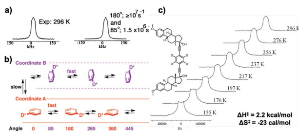
Fig. 19 (a) Quadrupolar echo ^2\text{H} NMR spectrum of molecular rotor 9 at 296 K and a simulated spectrum corresponding to a kinematic process that involves 180° rotations in the fast exchange regime ( >10^7 \text{ s}^{-1} ) combined with 85°/95° jumps in the intermediate exchange regime ( 1.5 \times 10^6 \text{ s}^{-1} ). (b) Representation of this process in terms of two coordinates that correspond to rotation in each of the two disordered sites, labelled as coordinate A and coordinate B. (c) Variable temperature ^2\text{H} NMR spectra corresponding to a process that retains fast 180° rotations and slow 85°/95° jumps varying from 2 \times 10^4 \text{ s}^{-1} at 155 K to 1.2 \times 10^6 \text{ s}^{-1} at 296 K, which reveal a low activation enthalpy and large and negative activation entropy (adapted from ref. 34).
