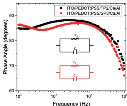
Fig. 6 Variation of phase angle depend on frequency for fabricated OLED device with TP2 and SP3. The inset shows electrical equivalent circuit model used for devices.
