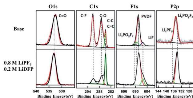
Fig. 6 C1s, O1s, F1s, P2p XPS spectra of cathode surface in base and dual-lithium salts electrolytes.
