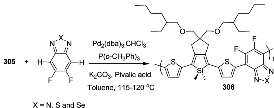
Scheme 86 Synthesis of 2,5-dithienylsilole–difluorobenzodiazine polymers 306a–c by DarP reaction.
