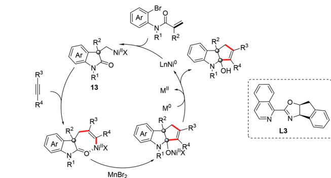
Scheme 11 Ni-Catalyzed enantioselective reductive cyclization of alkynes with arylbromide-tethered acrylamides.
