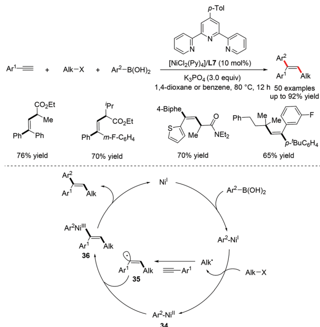
Scheme 22 Ni-Catalyzed anti -selective arylation of 2-alkynyl- N -sulfonylanilides.
