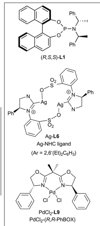
Scheme 15 Asymmetric conjugate additions with three different catalysts, to give different transformations, which have been successfully used in complex natural product synthesis. (A) (i) Synthesis of conidiogenol ( 9 ) via copper-catalyzed asymmetric conjugate addition of the methyl group to afford intermediate 101 . 82 (ii) Tandem copper-catalyzed asymmetric conjugate addition/enolate trapping with Stork–Ganem reagent ( 51 ) and subsequent condensation to give functionalized enone 35 in the synthesis of aflavazole ( 6 ). 51 (B) Palladium-catalyzed asymmetric conjugate addition of arylboronic acid 166 to enone 156 to generate \beta -aryl-substituted all-carbon quaternary stereocenter on 167 , which is an intermediate in the synthesis of mastigophorene A ( 17 ). 147 (C) Organocatalytic asymmetric conjugate addition of nitromethane to enone 173 produces a nitro-group-containing adduct 175 , which is used in the total synthesis of (–)-haliclونin A ( 18 ). 164
