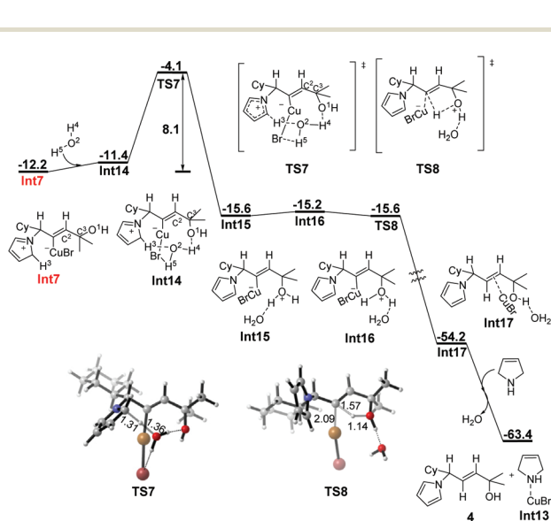
Fig. 3 Free energy profile ( \Delta G in \text{kcal mol}^{-1} ) for \text{H}_2\text{O} -assisted stepwise protodemetalation of Int7 . Bond lengths are given in angstroms.
