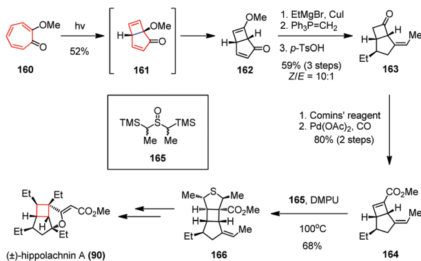
Scheme 23 4π electrocyclization in the total synthesis of (±)-hippolachnin A.
