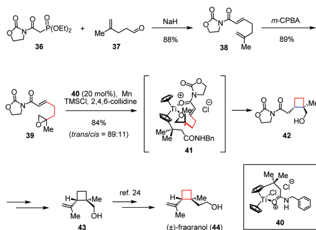
Scheme 6 \text{Ti(III)} -triggered 4- exo radical cyclization in the total synthesis of ( \pm )-fragranol.
