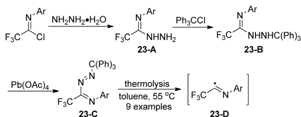
Scheme 23 Preparation and thermolysis of N -[2,2,2-trifluoro-1-(tritylazo)ethylidene]anilines.
