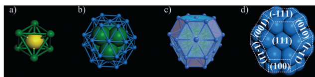
Fig. 4 (a) The central \text{Ag}_6 octahedron with a central sulfur; (b and c) the \text{Ag}_6\text{S}@\text{Ag}_{32} kernel; and (d) the crystal facets of the FCC \text{Ag}_{38} kernel. S yellow, Ag other colors. Adapted with permission from ref. 67. Copyright 2018, John Wiley & Sons, Inc.
