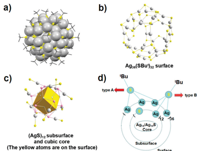
Fig. 3 X-ray structure of [\text{Ag}_{62}\text{S}_{13}(\text{S}'\text{Bu})_{32}]^{2+} . (a) The similar frameworks contained in the Ag-QD, Ag-inter, and Ag-NC. (b) \text{Ag}_{36}(\text{S}'\text{Bu})_{32} shell. (c) Bonding mode of core silver atoms (gray) and sulfur atoms (pink) linked with the shell sulfur atoms (yellow). (d) Two types of ligands. Adapted with permission from ref. 66. Copyright 2016, American Chemical Society.
