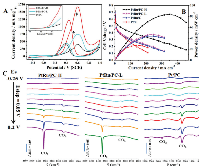
Fig. 2 (A) MOR in 0.5 M CH 3 OH + 0.1 M HClO 4 solution for PtRu/PC-H, PtRu/PC-L, and Pt/PC nanocatalysts at a scan rate of 50 mV s -1 . (B) Steady-state polarization and power density curves for fuel cells employing PtRu/PC-H, PtRu/PC-L, commercial PtRu/C, and commercial Pt/C as anode catalysts. (C) In situ FTIRS for methanol electrooxidation on three nanocatalysts, the reference spectra were acquired at -0.27 V. Reproduced with permission from ref. 89. Copyright 2019, Elsevier BV.
