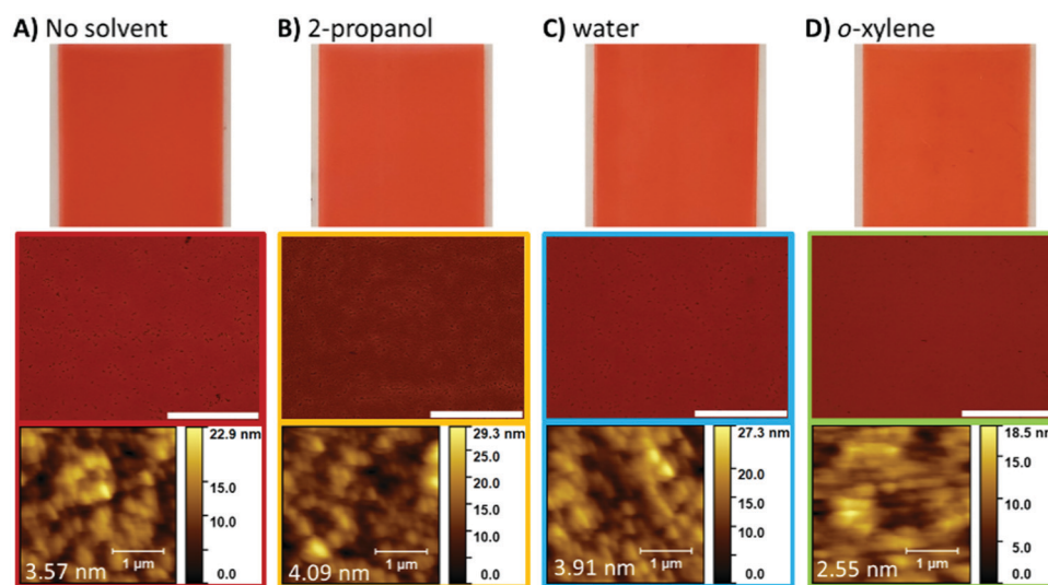
Fig. 6 Photographs of 1.5 \text{ cm} \times 1.5 \text{ cm} (top), optical microscopy images ( 10\times magnification with white scale bar corresponding to 500 \text{ }\mu\text{m} ) (middle), and atomic force microscopy height images along with the corresponding root mean square roughness RMS (bottom) for PDIN-H films on PET (A) as-cast with no solvent coated on top and with (B) 2-propanol, (C) water, or (D) o -xylene slot-die coated on top and left to dry. PDIN-H films were formed via slot-die coating 10 \text{ mg mL}^{-1} PDIN-H solutions in 1-propanol with 1 molar equivalent of NaOH added.
