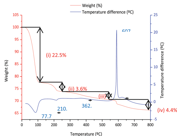
Fig. 5 TGA and DTA analysis of the 80 °C-12 h dried 80 \text{SiO}_2 :20 \text{LaF}_3 particulate sol.
