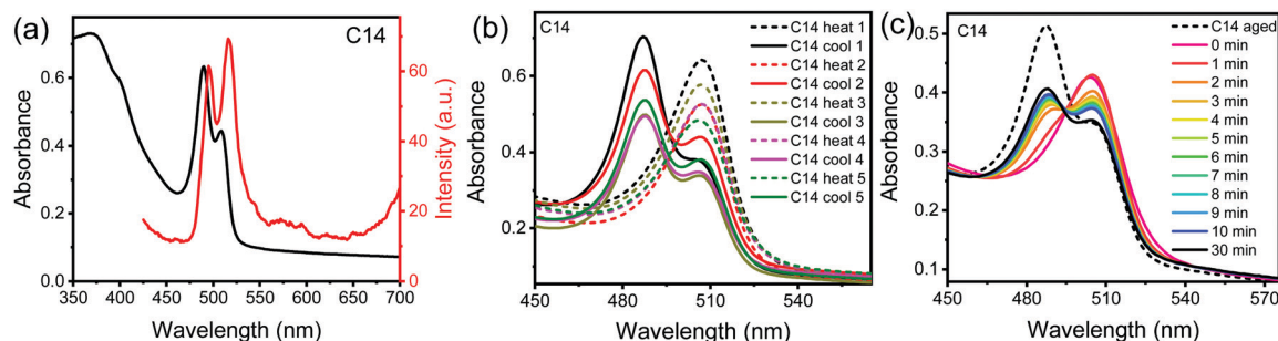
Fig. 2 (a) Absorption and photoluminescence spectra of (C 14 H 29 NH 3 ) 2 PbI 4 2D perovskite thin films. (b) Absorption spectra of (C 14 H 29 NH 3 ) 2 PbI 4 2D perovskite thin film recorded just after annealing the thin film at 100 °C (dotted curve) and thin film cooled to room temperature for 1 h (solid curve). (c) Evolution of absorption spectra of (C 14 H 29 NH 3 ) 2 PbI 4 2D perovskite thin films just after annealing at 100 °C with time.
