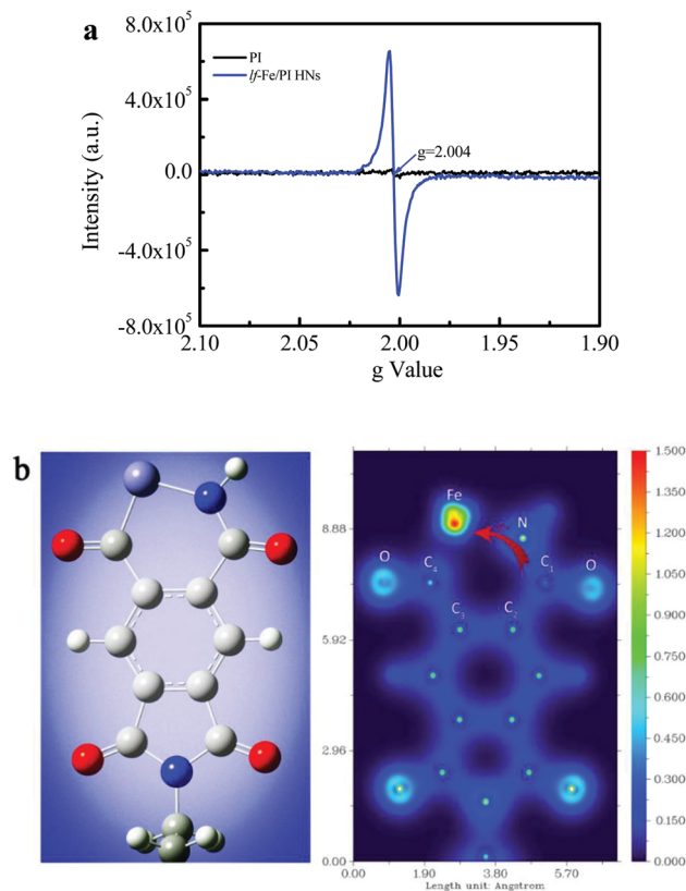
Fig. 4 Non-uniform distribution of surface electrons on If-Fe/PI HNs. (a) EPR spectra of PI and If-Fe/PI HNs. (b) DFT calculations for the optimized structure of If-Fe/PI HNs in one unit (left) and the corresponding two-dimensional valence-electron density color-filled maps of the If-Fe/PI HNs model (right). Purple, red, grey and blue circles denote Fe, O, C and N atoms, respectively. The valence-electron density is given in \text{e} \text{Å}^{-3} .
