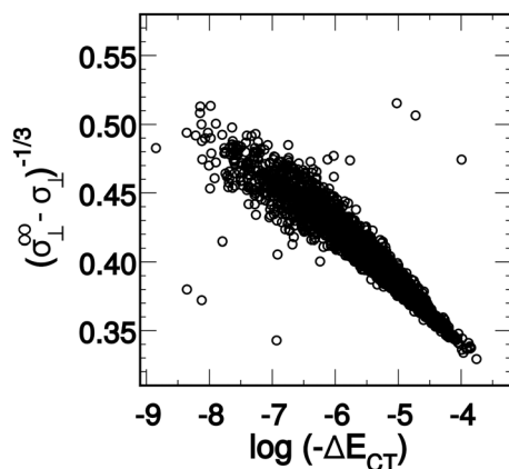
Fig. 1 A derived linear model relating the orthogonal component of the ^1\text{H} shielding tensor in water ( \sigma_{\perp}^{\infty} ) to the stabilization energy due to charge-transfer ( \Delta E_{\text{CT}} ). The shielding tensor component in the limit of a HB-free water molecule is denoted as \sigma_{\perp}^{\infty} . Reproduced from ref. 17/CC BY.
