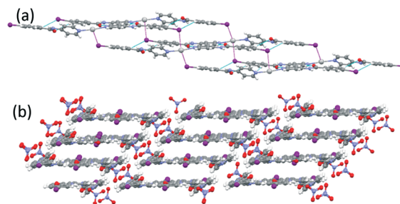
Fig. 5 A view showing \text{C}-\text{I}\cdots\text{Ag} interactions in violet (a) and nitrate anion linking planes by \text{C}-\text{I}\cdots\text{O} halogen bonding and \text{Ag}\cdots\text{O} interactions (b) in 1 .
