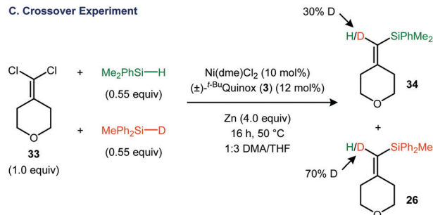
Fig. 4 Mechanistic studies using a deuterium-labelled silane.
