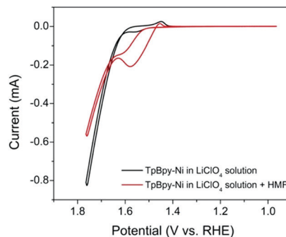
Fig. 4 CVs of TpBpy-Ni@FTO in the absence (black line) and in the presence (red line) of 5 mM HMF in 0.1 M \text{LiClO}_4 solution (pH = 13).
