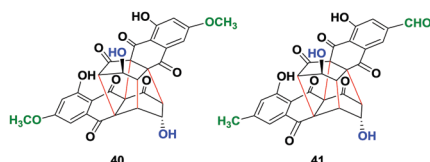
Fig. 2 Rugulin analogues (40 &amp; 41) synthesized by the oxidation of rugulosin analogues using ceric ammonium nitrate (CAN) in water.
