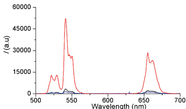
Fig. 1 PL intensity spectra of c-UCNP upon excitation at 980 nm (black), css-UCNP upon excitation at 980 nm (red), and css-UCNP upon excitation at 808 nm (blue). All UCNPs were conjugated with ssDNA and had a concentration of 10 \text{ mg mL}^{-1} in water. The excitation power was constant for all PL spectra ( P = 223 \text{ } \mu\text{W cm}^{-2} ).
