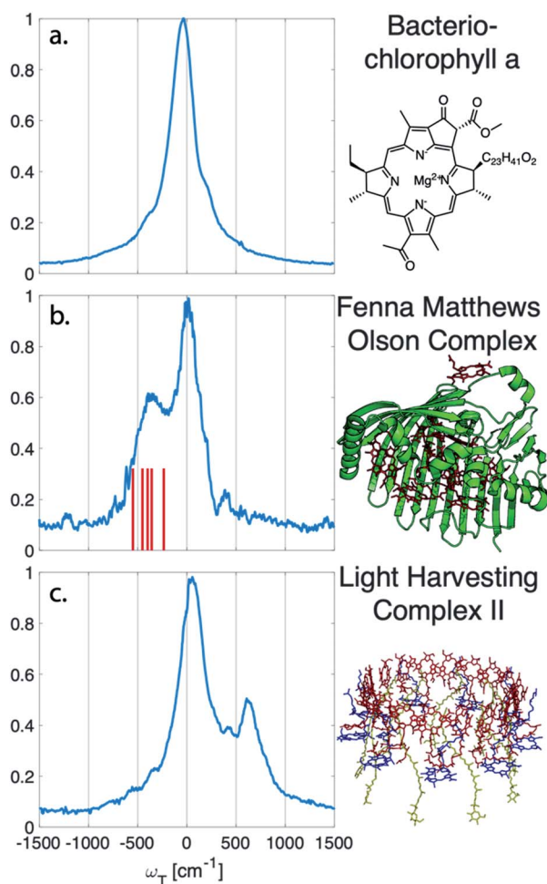
Fig. 2 Sum of the electronic coherences over the entire 2D spectrum. (a) The BChla spectra contains only vibrational coherences. With the long-lived coherences subtracted, no additional peaks are observed. Both (b) FMO and (c) LH2 have multiple electronic states within the bandwidth of the pulse and display fast decaying coherences. For FMO, excitonic energy level differences are drawn as a stick spectrum for differences between 330–550 \text{cm}^{-1} . The closest excitonic energy level difference to the main peak is between excitons 7 and 2 at 400 \text{cm}^{-1} , with the energy levels taken from ref. 22.
