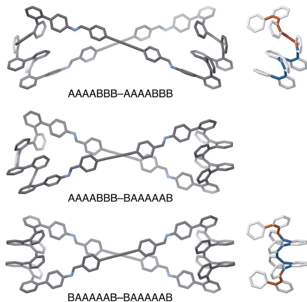
Fig. 10 Left: Optimized geometries (PCM( \text{CHCl}_3 )/B97-D/cc-pVDZ) of \text{oP}^{10}(\text{DPB})_{2+2} in its homochiral-antiparallel-(AAAABBB) 2 (top), homochiral-(AAAABBB)(BAAAAAB) (middle), and homochiral-(BAAAAAB) 2 (bottom) configurations. Right: o -phenylene geometries with the A...A (blue) and B...B (orange) folding states highlighted on the backbone.
