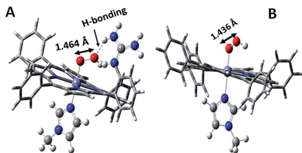
Fig. 9 DFT optimized structures of N -methylimidazole bound (A) protonated \text{Fe}^{\text{III}}\text{-MARG} hydroperoxide and (B) \text{Fe}^{\text{III}}\text{-TPP} hydroperoxide.
