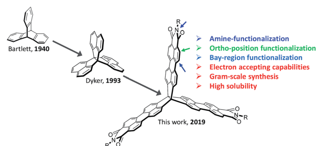
Fig. 1 Representation of the structural evolution of 3D-symmetric building blocks for rigid 3D PAHs, from triptycene (left) to triphenylene (middle) to triperylene[3,3,3]propellane triimides (right).
