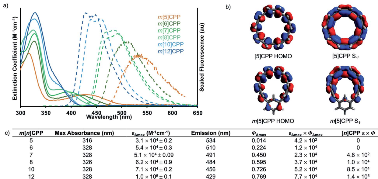
Fig. 3 (a) Absorbance and emission spectra of m [ n ]CPPs; (b) HOMO (left) and S 1 ' (right) orbital depiction of [5]CPP and m [5]CPP, demonstrating change in orbital symmetry. Calculated using CAM-B3LYP/STO-3G level of theory; (c) absorbance, extinction coefficient ( \epsilon ), emission and quantum yield ( \Phi ) of m [5]– m [8]-, m [10]- and m [12]CPP and brightness comparison of m [ n ]CPPs and [ n ]CPPs.
