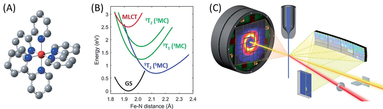
Fig. 1 The [Fe(bpy) 3 ] 2+ complex under investigation, Fe (red), N (blue), C (grey), H not shown (A), its most important ground and excited state potential energies as a function of Fe–N bond length (B) from Sousa et al. 35 and the experimental setup (C).
