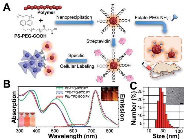
Fig. 1 (A) Schematic illustration of the preparation of carboxyl-functionalized Pdotes through nanoprecipitation and subsequent bioconjugation for in vitro specific cellular imaging and in vivo tumor targeting. (B) Absorption spectra of PF-TFQ-BODIPY Pdotes (solid green line), TPE-TFQ-BODIPY Pdotes (solid blue line), and Pttc-TFQ-BODIPY (solid red line) in water. Their corresponding emission spectra are shown with dashed lines. The insets in the bottom-left and upper-right corners show the photographs of the Pdote solutions (from left to right: PF-TFQ-BODIPY, TPE-TFQ-BODIPY, and Pttc-TFQ-BODIPY Pdotes) under daylight and under UV light illumination, respectively. (C) Hydrodynamic diameters of Pttc-TFQ-BODIPY Pdotes measured by dynamic light scattering. The inset shows the transmission electron microscopy image of Pttc-TFQ-BODIPY Pdotes. Scale bar is 100 nm.
