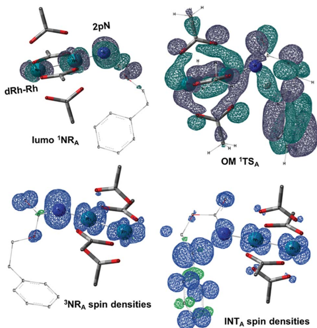
Fig. 7 LUMO of the singlet nitrene species (LUMO 1 NRA), the density of the unpaired electrons of the triplet nitrene species ( 3 NRA spin densities), the frontier orbital of 1 TS A (OM 1 TS A ) and the spin densities of the diradical intermediate (INT A ). (Different atom styles are used for clarity.)
