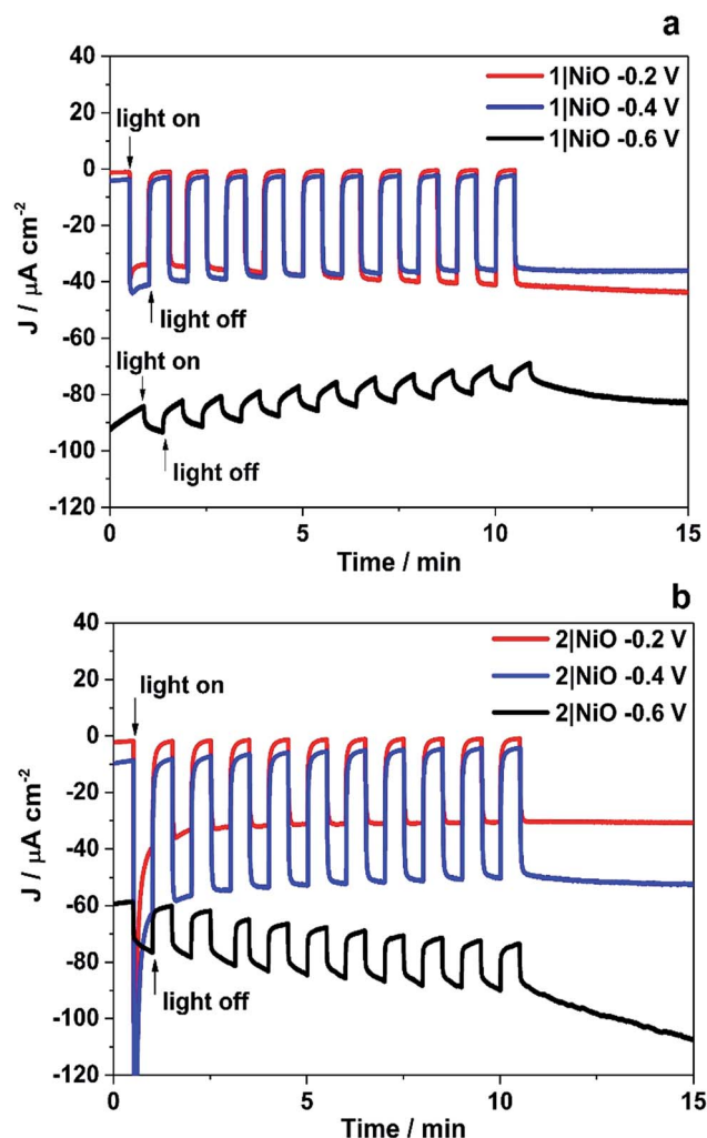
Fig. 7 Chronoamperometry measurements of 1|NiO (a) and 2|NiO (b) immersed in pH 3 buffer containing 0.1 M potassium hydrogen phthalate. E_{\text{appl}} = -0.2\text{ V} , -0.4\text{ V} and -0.6\text{ V} vs. Ag/AgCl (3.0 M NaCl). Chopped light illumination was applied with 30 s intervals (10 cycles of dark current/photocurrent).
