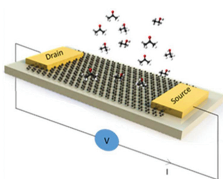
Fig. 5 A schematic design of the flat or patterned MLG-based sensors for E/I/A-containing cancer marker detection. Graphene is placed on a flexible PVC substrate of 25 \mu\text{m} thickness. A two-point measurement concept was used for the in situ electrical characterization of CM-induced graphene electrodes and its selectivity analysis.
