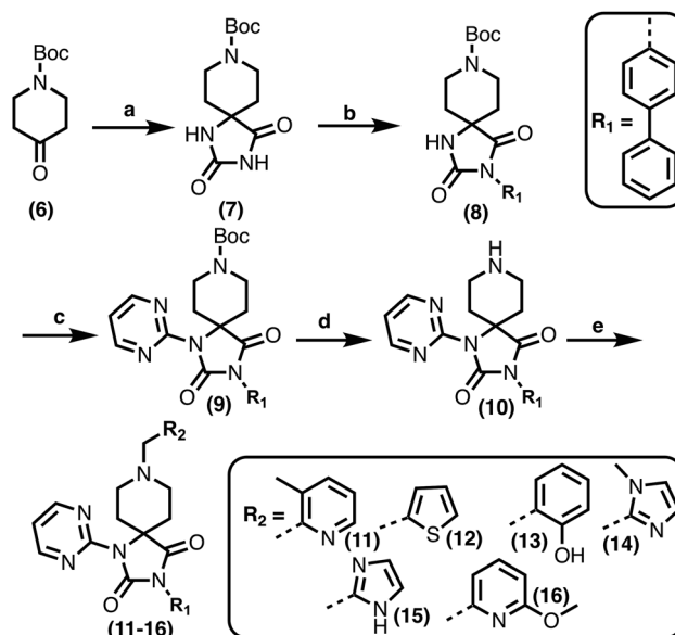
Fig. 3 Synthesis of 3-((1,1'-biphenyl)-4-yl)-8-((aryl)-1-(pyrimidin-2-yl))-1,3,8-triazaspiro[4.5]decanone-2,4-dione compounds ( 11-16 ) to investigate the role of the pyrimidine group in tPHD2 inhibition. Conditions: a) KCN, NH 4 CO 3 , EtOH:H 2 O (1:1), 60 °C; b) CuI, K 2 CO 3 , 4-iodobiphenyl, N,N -dimethyl-ethylenediamine, ascorbate, DMF, CH 3 CN (1:1), reflux; c) 2-iodopyrimidine, CuI, TMHD, Cs 2 CO 3 , DMF:CH 3 CN (1:1), reflux; d) HCOOH, rt, 3 h; e) RCHO, NaBH(OAc) 3 , HCOOH. R 1 = biphenyl.
