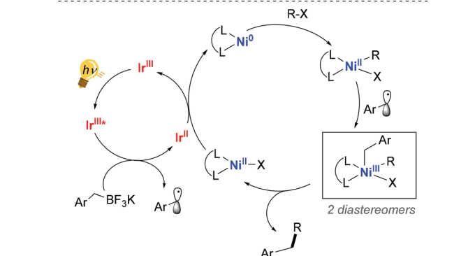
Scheme 8 Photoredox/Ni dual catalytic cross-coupling (top) and mechanism (bottom). Reagents and conditions: organoboron racemic mixture 17 (1.20 equiv.), aryl bromide 18 (1.00 equiv.), 2,6-lutidine (3.50 equiv.), Ir-photocat. (2.0 mol%), Ni-cat. (3.0 mol%), chiral ligand (3.0 mol%), THF/MeOH (95/5), blue LED, 24 h. 58
