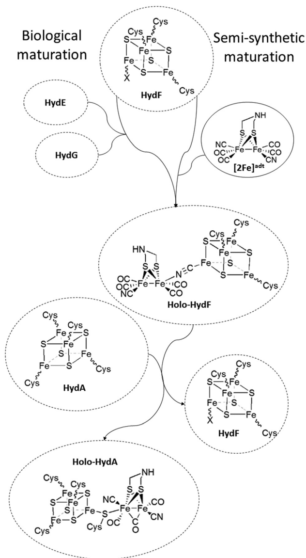
Fig. 1 Schematic representation of the assembly of holo-HydF ( [2Fe]^{adt} -HydF) and formation of the H-cluster. During the biological process, a pre-catalyst is assembled on HydF through the activities of HydE and HydG. In the semi-synthetic route, holo-HydF is generated via the incorporation of synthetic mimics of the [2Fe] subsite.
