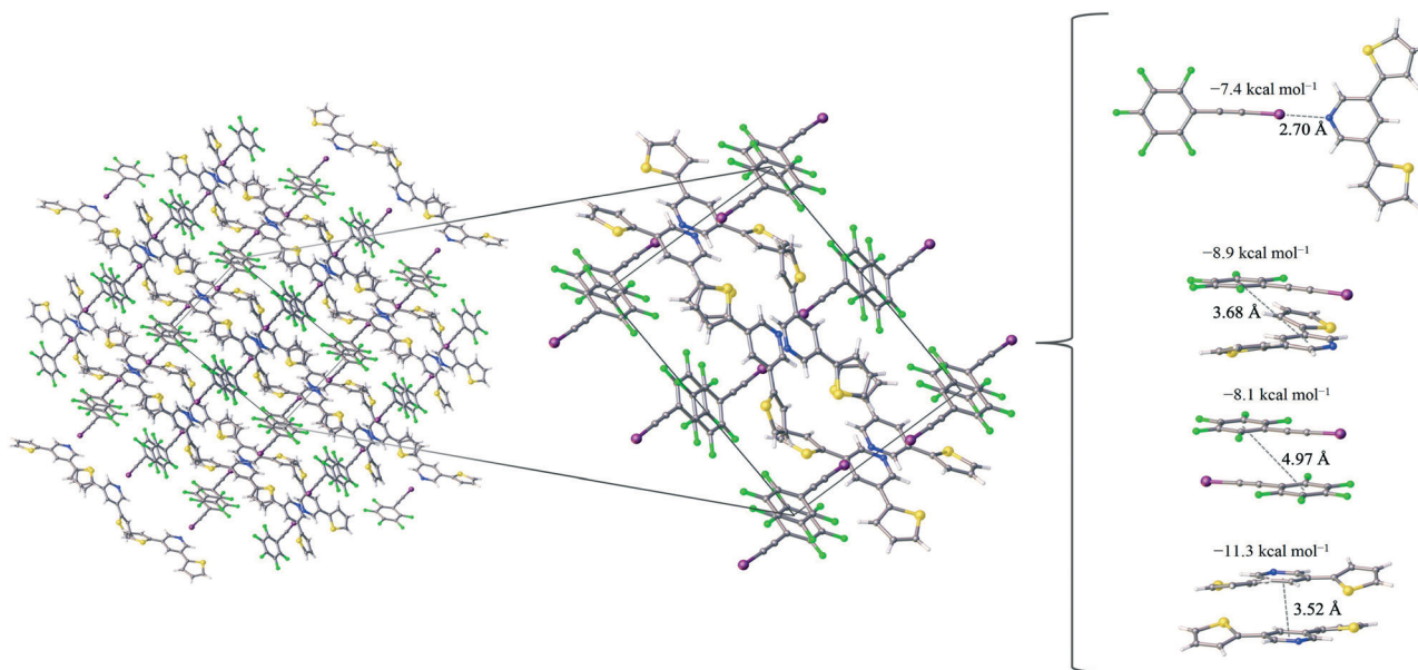
Fig. 3 The F_5BAI - PyrThio_2 co-crystal, a zoomed in picture of the unit cell which shows the presence of non-covalent interactions as well as the pair-wise contacts with the largest interaction energies labeled with the corresponding distance (in Å) and the average interaction energy (in kcal mol ^{-1} ).
